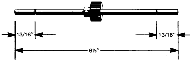
P017—PINION FOR CA HEAD 6 1/8" LONG
