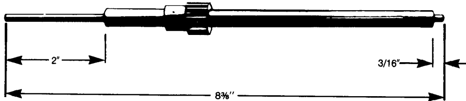
P033—PINION FOR C HEAD 8 3/8" LONG
